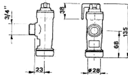
FLUXOR INODORO PALANCA S/REGUL emp 400.14
