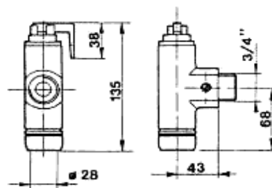
FLUXOR INODORO PALANCA C/REGULemp 400.07
