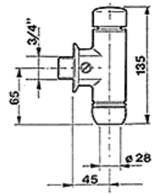
FLUXOR INODORO 3/4 C/REGUL tubo 26x28 400.01
